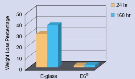
Weight loss comparison of E-glass and E6 ® fibers soaking in 10% H 2 SO 4 solution at 96°C after 24 hours and 168 hours
